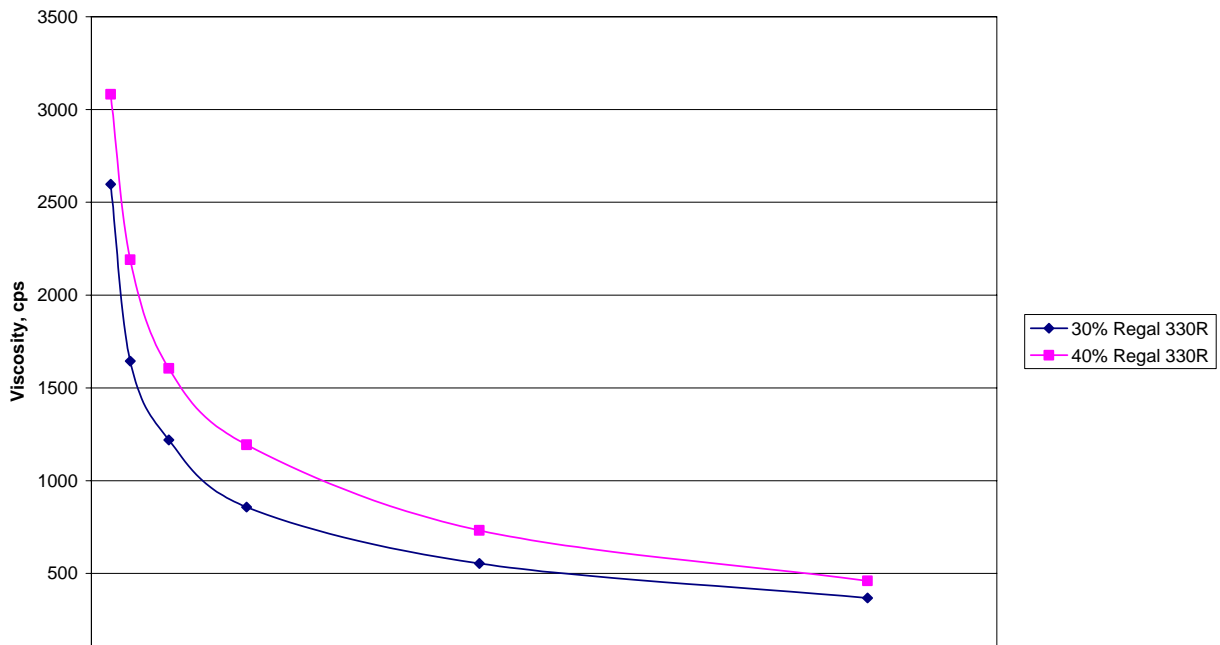
Dispersion Viscosities
